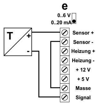
Temperature Sensor with Two-wire Current Loop Transducer
