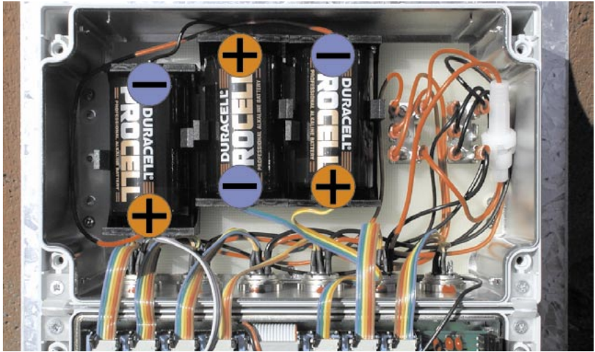
Internal Batteries
